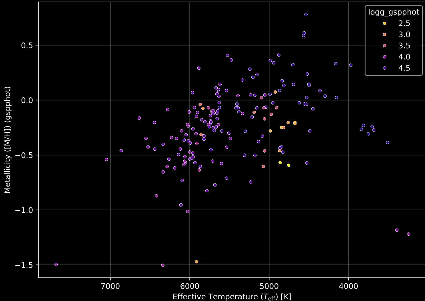
APOGEE DR17 Field: [115+69_MGA] Stellar Population Parameters (n= 177)
