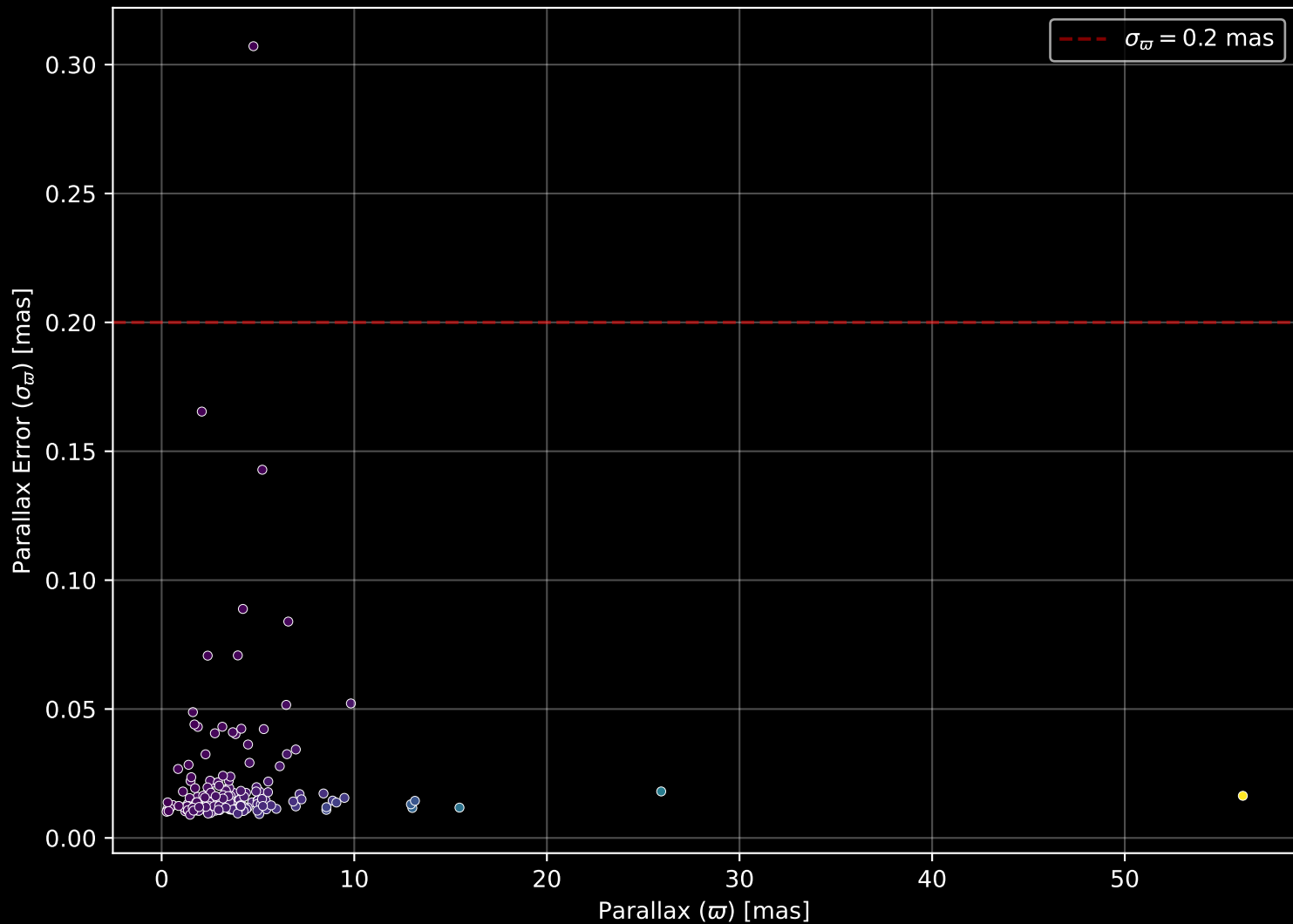
APOGEE DR17 Field: [115+69_MGA] Parallax Quality (n= 177)
